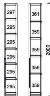
Höhe "4" 2000 mm
