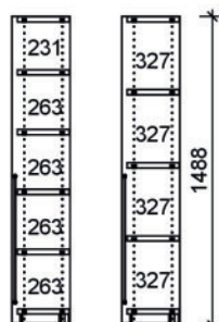
Höhe "2" 1488 mm
