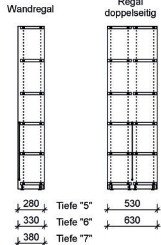
Höhe "4" 2000 mm
