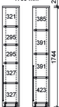
Höhe "3" 1769 mm
