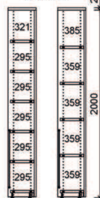
Höhe "4" 2025 mm
